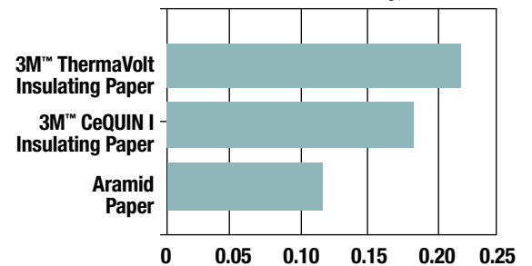
Varnish Absorption
