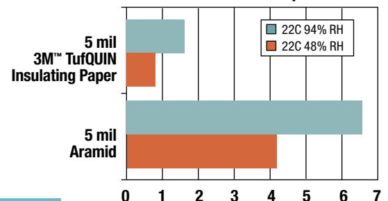
Moisture Absorption
