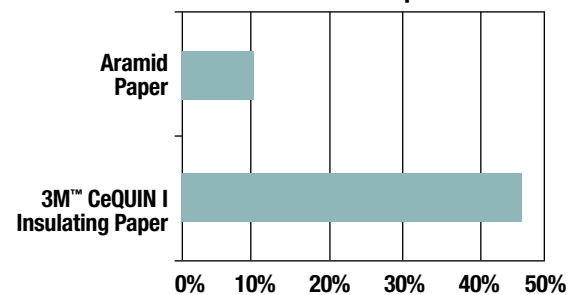
Moisture Absorption
